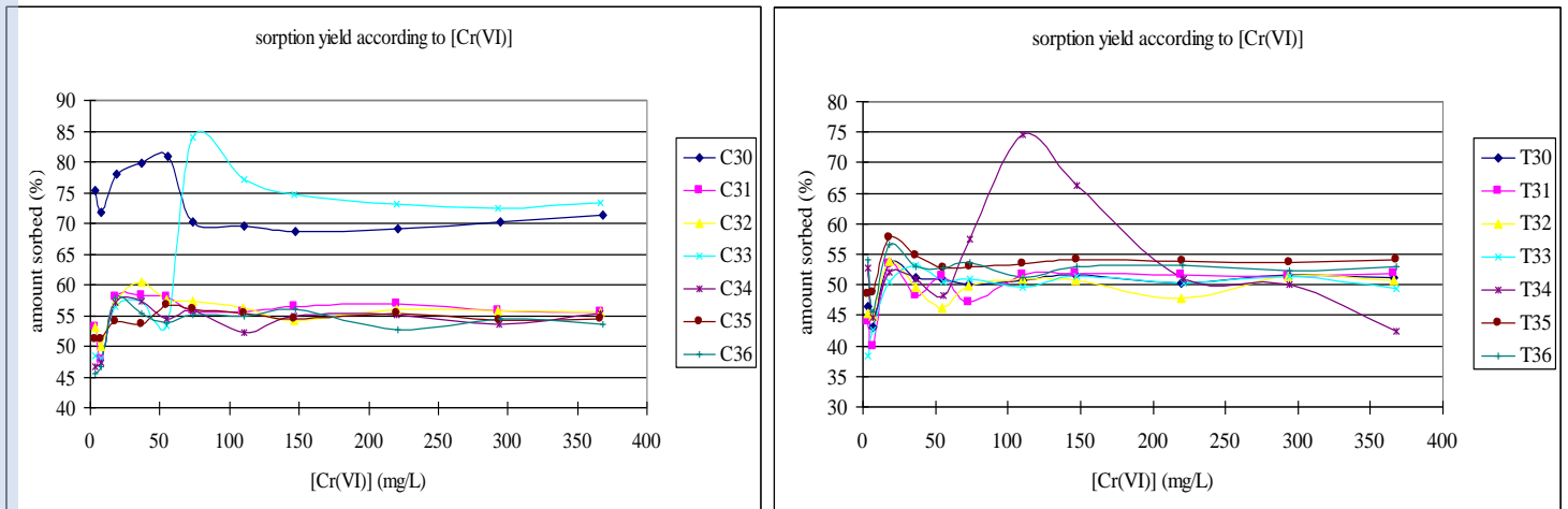
Figure 6 : sorption yield according to [\text{Cr}^{\text{VI}}] for the big bag 3
