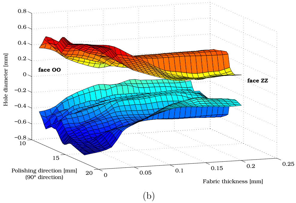
Figure 16: 3D reconstruction of a stitching hole in Automotive [0/90] NC2 : view (a) from the zig-zag face and (b) from the side.
