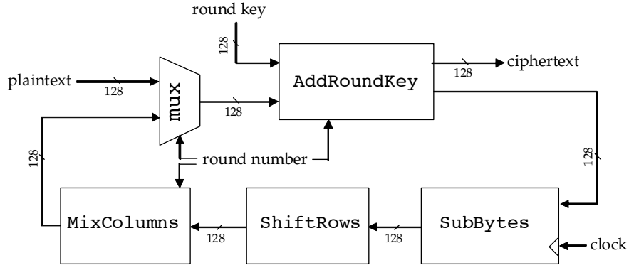
Fig. 5. AES Structure
