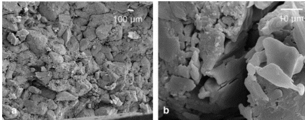
Figure 8: Fractured face of a tablet made at room temperature.
