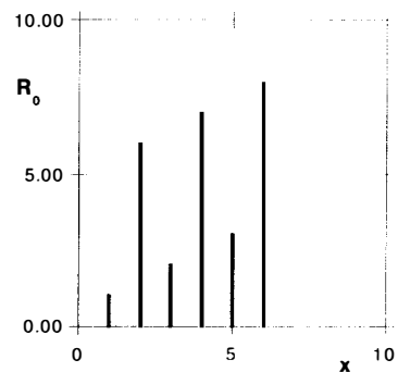
Fig. 7. Initial particles arrangement defined by R_0[2i+1] = i+1 ; R_0[2i+2] = (N/2) + i+1 ; 0 \leq i \leq (N/2) - 1 .
