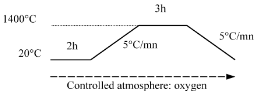
Figure 1: Thermal cycle for the treatment of the \alpha -Al 2 O 3 -ZrO 2 mixtures.
