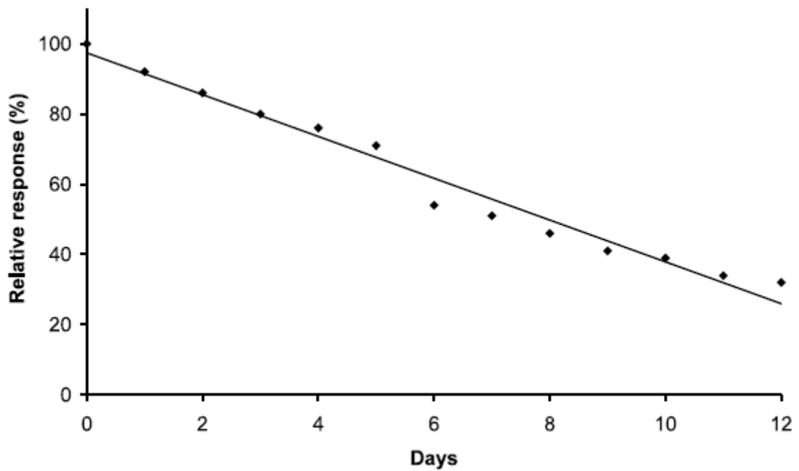
Figure 5: Long-term stability of a PEDT/PPO electrode using preparation method A. Conditions: 5 \mu\text{M} catechol, 0.1 M, pH 6.5 sodium phosphate buffer and 0.1 M KCl, 25 ^{\circ}\text{C} , -/200 mV vs. SCE.
