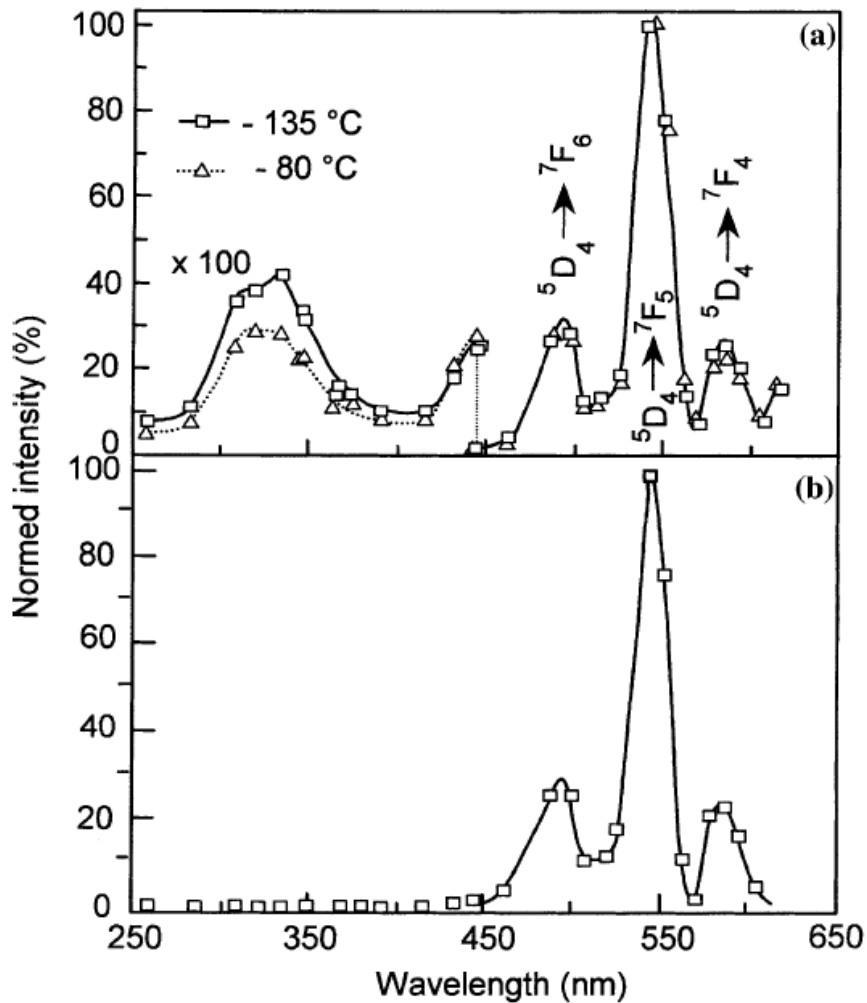
Figure 2: Spectral distribution of: (a) -135^\circ\text{C} and -80^\circ\text{C} TL peaks of \text{LaCeT} ; and (b) \text{La}_{0.86}\text{Tb}_{0.14}\text{PO}_4 samples obtained after X-ray irradiation at LNT (0.35 Gy).
