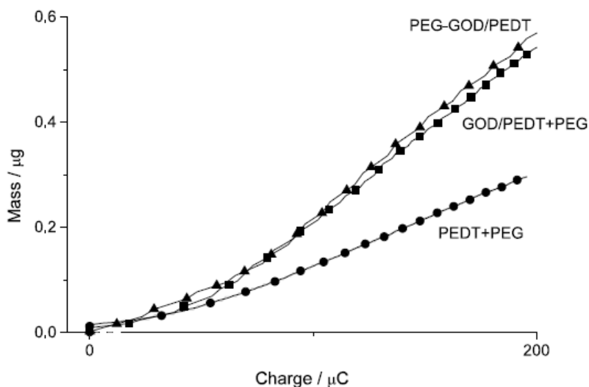
Figure 4: Data from ECQM: electrode mass versus charge during the potentiostatic electrosynthesis of (a) (PEDT+PEG) film ( \bullet ), (b) (GOD/PEDT+PEG) film ( \blacksquare ) and (c) (PEG-GOD/PEDT) film ( \blacktriangle ). Quartz surface: 0.2 \text{ cm}^2 . Films were grown until a charge of 200 \mu\text{C} was reached, in 0.05 \text{ M} phosphate buffer (pH 6) containing 0.05 \text{ M KCl} + 10^{-2} \text{ M EDT} + 10^{-4} \text{ M PEG} (a), 10^{-4} \text{ M PEG} + 1000 \text{ IU ml}^{-1} \text{ GOD} (b) or 10^{-4} \text{ M PEG} + 1000 \text{ IU ml}^{-1} \text{ PEG-GOD} (c).
