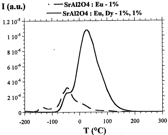
fig.9 : Dy co-activation influence on the TL curves
