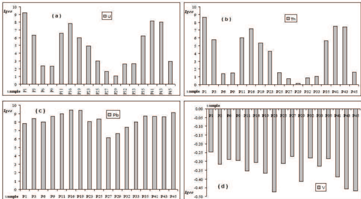
Figure 3. The geo-acumulation index in bottom sediments: (a) U; (b) Th; (c) Pb; (d) V.
