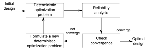
Figure 6: SORA procedure [41]
