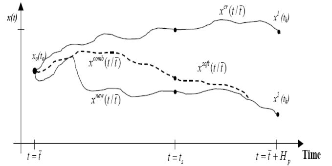
Fig. 6. Soft switching.
