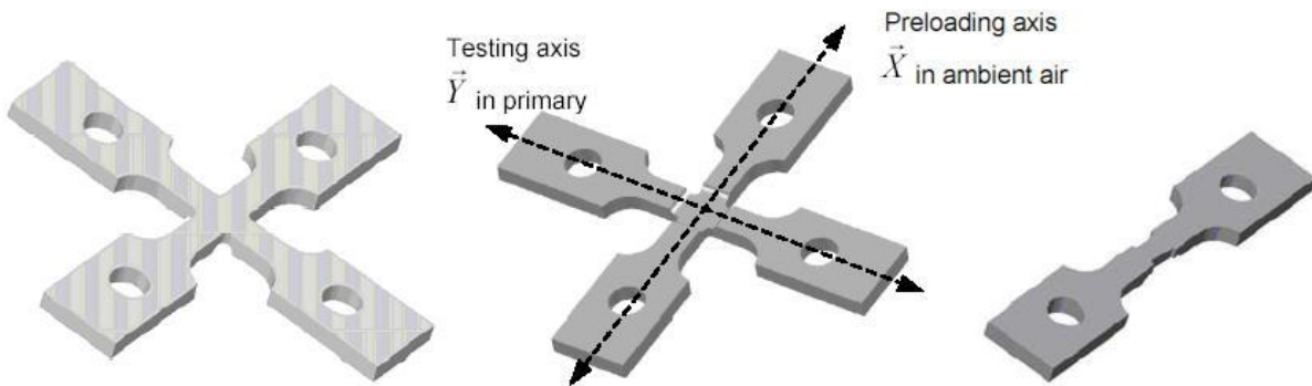
Figure 1 – Cross-shaped specimen
