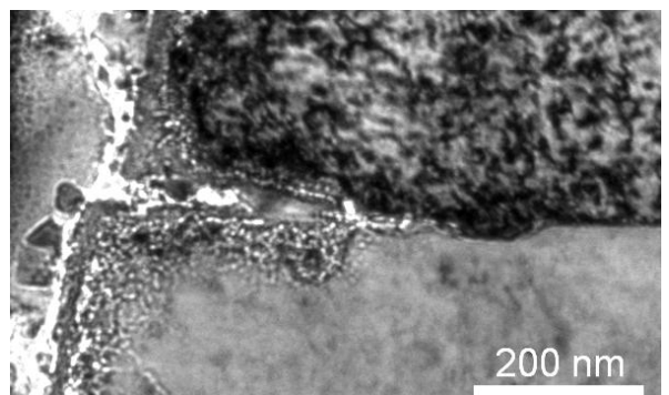
Figure 25 – Different dislocation densities between grains. Defocused bright field image of the crack initiated at site 3 of specimen T217-01
