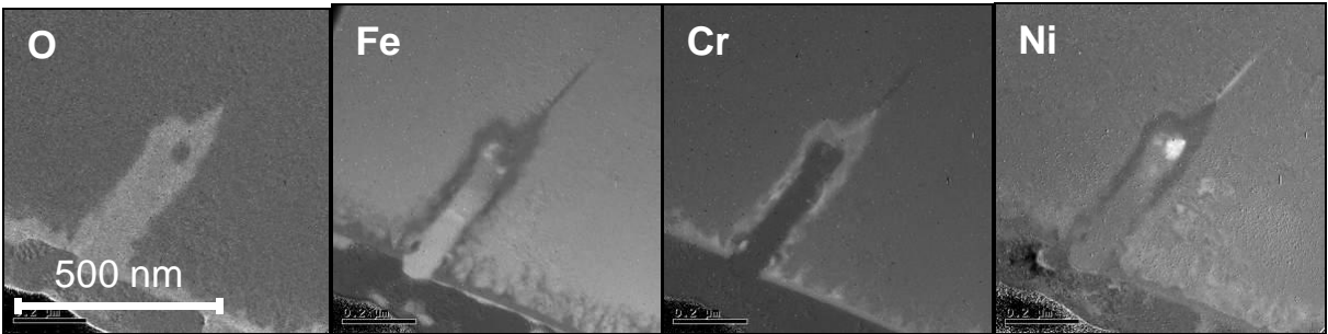
Figure 27. O, Fe, Cr and Ni EFTEM maps of the crack initiated at site 2 on T217-01
