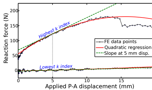
Figure 6. Reaction force of the tibia along the P-A direction vs. applied P-A drawer: joint stabilizing effect of simulations A and B (maximum and minimum stiffness indexes). The response of the limb only has been subtracted.
