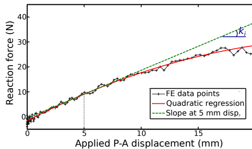
Figure 5. Reaction force of the tibia along the P-A direction vs. applied P-A drawer magnitude to determine k .
