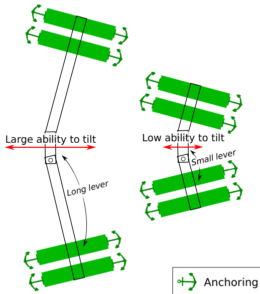
Figure 10. Mechanism explaining the advantage of small braces to prevent drawer.
