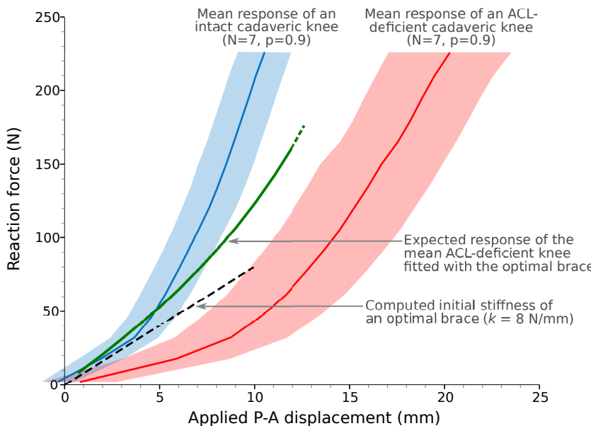
Figure 11. Quantification of the additional stiffness brought by an optimal brace ( k = 8 \text{ N/mm} ) to an ACL-deficient cadaveric knee under a P-A displacement. Data kindly provided by Eagar et al. (2001).
