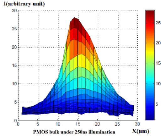
Figure 9: Induced current of 28nm bulk PMOS under illumination of 500ns and 250ns
