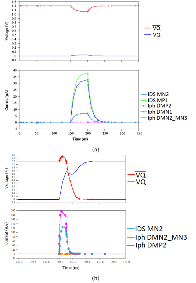
Fig. 12: Extracted waveforms from the electrical simulator at the drain of MP2 for (a) 50 ns [9] and (b) 30 ps pulse duration.
