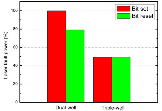
Figure 3. Comparative study of the laser sensitivity threshold of a flip-flop in dual-well and triple-well.
