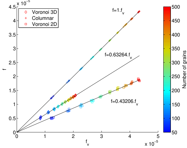
Fig. 4. Weighting coefficient of the homogeneous diffusivity as a function of the volume fraction of grain boundary.
