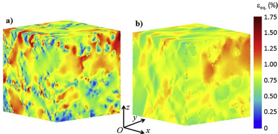
Fig. 14. Distribution of the equivalent plastic strain in the model with (a) complex IM 3D structure and (b) in the simplified “particle reinforced” composite. The distributions correspond to an overall tensile strain of 0.5% applied in the Oz direction.
