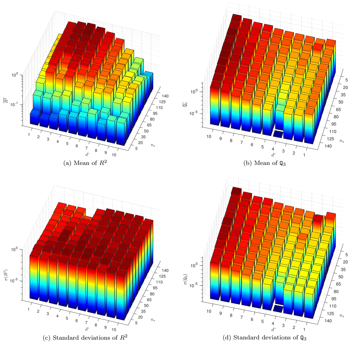
Figure 17: Performance of the LS metamodel in approximating the 5 dimensional Rosenbrock's function in terms of the number of sample points ( n_s ) and the degree of the polynomial ( d^\circ ).
