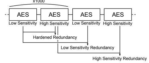
Fig. 5: Testing Procedure
