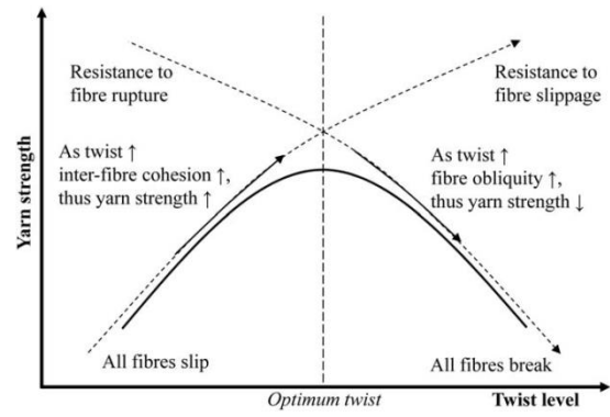
Figure 8. Fibre spinning (left) [147]. Right: Typical effect of twist on yarn strength [128].
