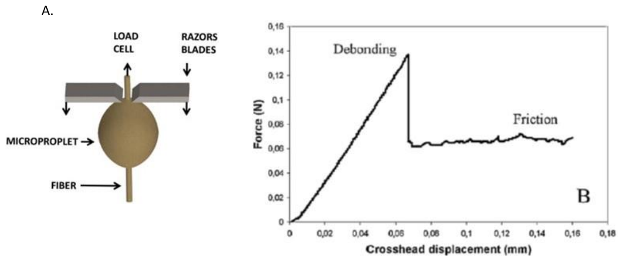
Figure 16. (Left) Schematic diagram of microdroplet test [190], (Right) Typical debonding behaviour [192]
