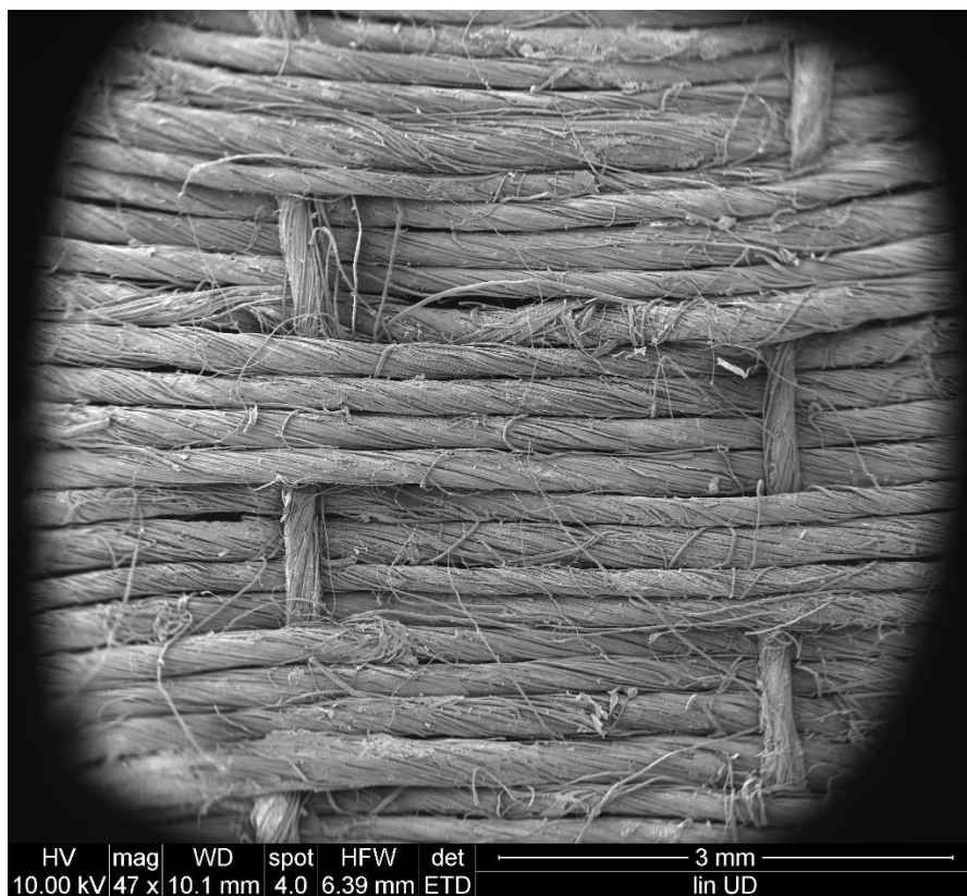
Figure 2 : Quasi-unidirectional flax preform made up of twisted fibre assemblies.
