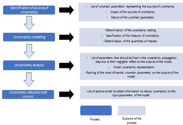
Fig. 1. Framework workflow.
