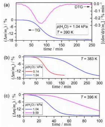
Figure 1. Specific features of isothermal mass-loss behavior of the thermal decomposition of \text{Cu(OH)}_2 in flowing \text{N}_2\text{-H}_2\text{O} mixed gas: (a) TG–DTG curves recorded at 390 K at p(\text{H}_2\text{O}) = 1.04 kPa, (b) a comparison of TG curves recorded at 383 K under p(\text{H}_2\text{O}) = 0.14 and 1.04 kPa, and (c) a comparison of TG curves recorded at 396 K under p(\text{H}_2\text{O}) = 1.04 and 9.59 kPa.
