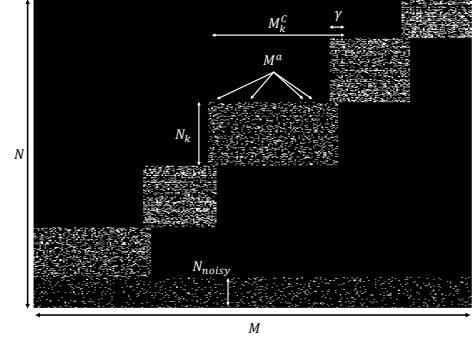
Fig. 1: Example of generated data. Here, \kappa = 5 , \alpha = 0.05 , \beta = 2 and \gamma = 0.1 , leading to \tilde{S} = 0.9 with each white pixel being a value of 1 and black pixels being a value of 0.
