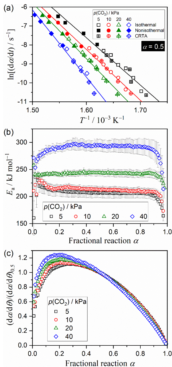
Figure 7. Results of the isoconversional kinetic analysis for the thermal decomposition of the ZnCO 3 sample under the individual conditions in a flow of N 2 -CO 2 mixed gas with various p(CO_2) values: (a) Friedman plots at \alpha = 0.5 , (b) E_a values at various \alpha values, and (c) experimental master plots of (d\alpha/d\theta)/(d\alpha/d\theta)_{0.5} versus \alpha .
