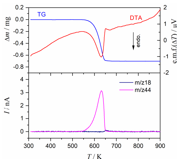
Figure 1. Typical TG/DTA-MS traces for the thermal decomposition of the \text{ZnCO}_3 sample.
