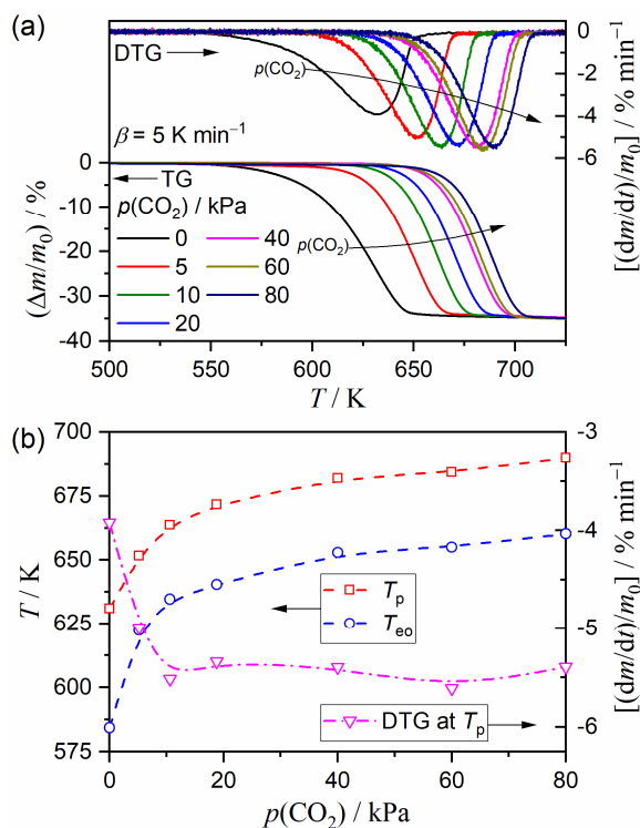
Figure 5. TG–DTG curves for the thermal decomposition of the ZnCO 3 sample ( m_0 = 5.056 \pm 0.103 mg) recorded at \beta = 5 \text{ K min}^{-1} in a flow of N 2 –CO 2 mixed gas with different p(\text{CO}_2) values (flowrate: 300 cm 3 min -1 ).
