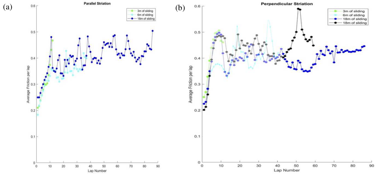
Figure 6: Evolution of the average COF, (a) Disc D//, (b) Disc D \perp
