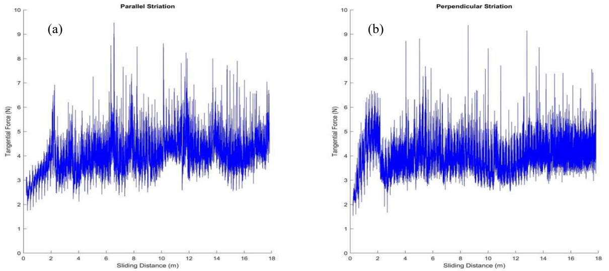
Figure 5: Evolution of the tangential force over time, (a) Disc D II (test 1), (b) Disc D I (test 4)
