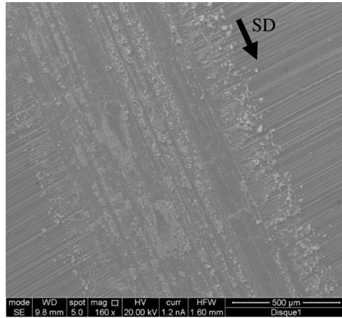
Figure 17: Disk D \perp (18m of sliding) SE image
