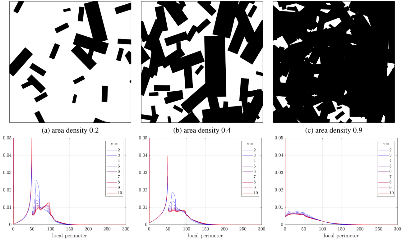
Fig. 3: (1st row) Samples of BMs of rectangles with fixed elongation ratio e = 3 . (2nd row) Probability density functions of the local perimeter measure of BMs of rectangles with the growing typical grain elongation ratio. The distributions are normalized by the total number of samples and the bin width.
