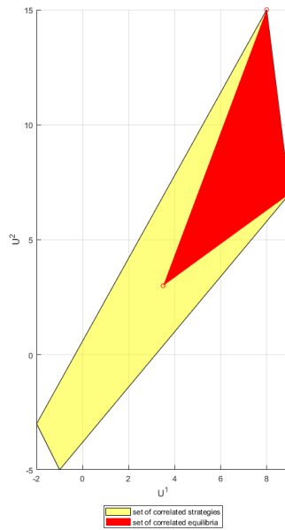
Fig. 4: Set of correlated strategies and correlated equilibria [27]
