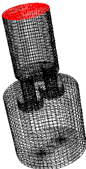
Figure 3 : mesh of RH + ladle reactor
