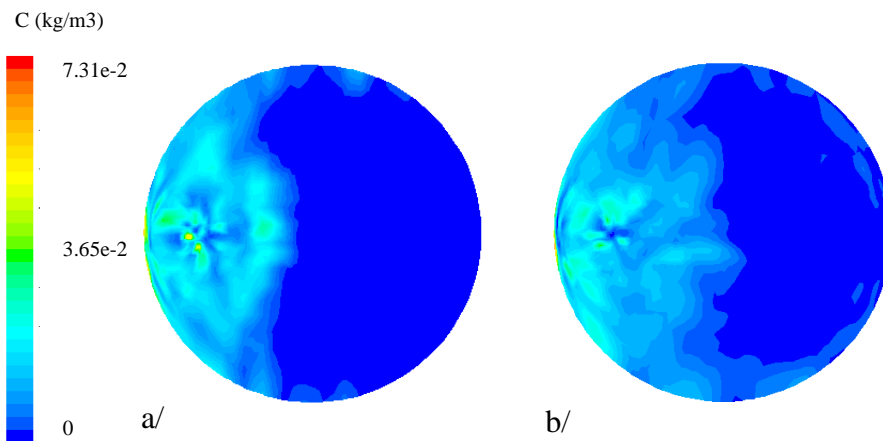
Figure 7: Bubble concentration at RH free surface - a : without bubble growth - b : with bubble growth.
