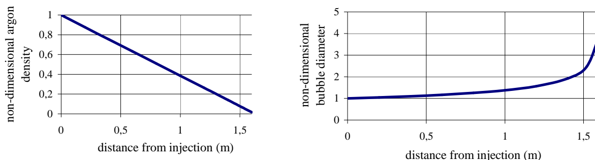
Figure 4 : Dependence of bubble properties on vertical position.
