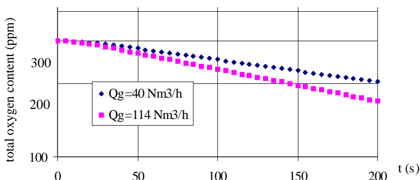
Figure 12 : Time evolution of total oxygen content
