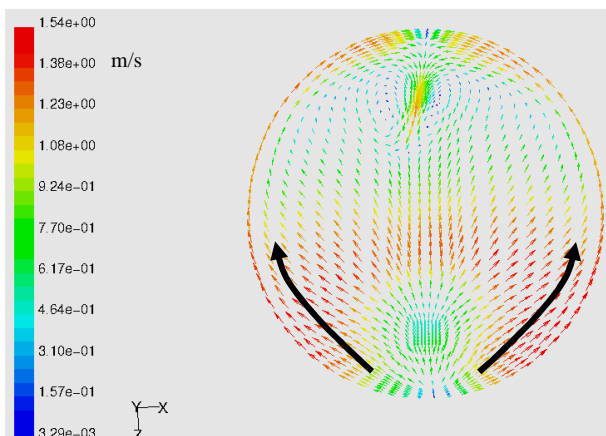
Figure 8 : Velocity field at RH free surface - top view.
