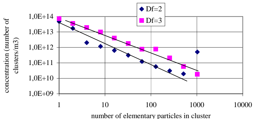
Figure 11 : Influence of fractal dimension ( t=100s ) - Q_g=130.1 \text{ Nm}^3/h - b=10^{-10} \text{ m} and t=100 \text{ s}
