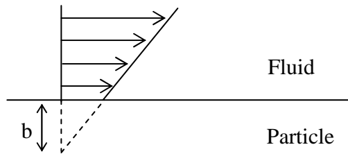
Figure 2 : fluid behaviour for hydrophobic surface
