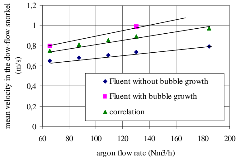
Figure 5 : Comparison of Fluent's results with standard correlation.
