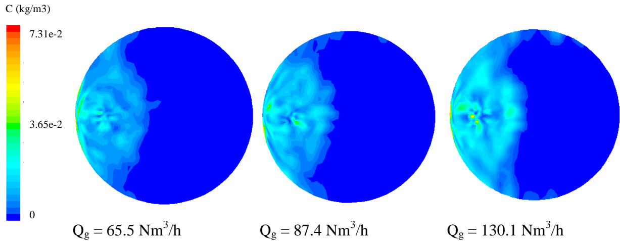
Figure 6 : Bubble concentration at degasser free surface - without bubble growth.
