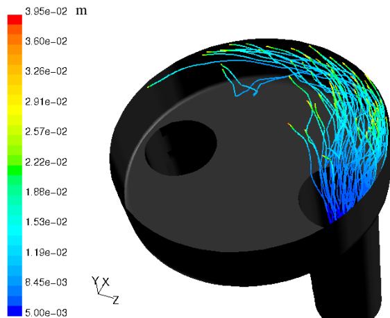
Figure 9 : Bubble trajectory, coloured by bubble diameter - Q_g=130.1 \text{ Nm}^3/\text{h} .
