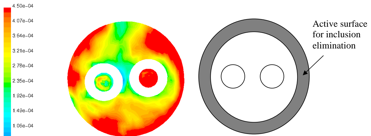
Figure 10 : Inclusion concentration under ladle free surface - Q_g=130.1 \text{ Nm}^3/\text{h} with bubble growth
