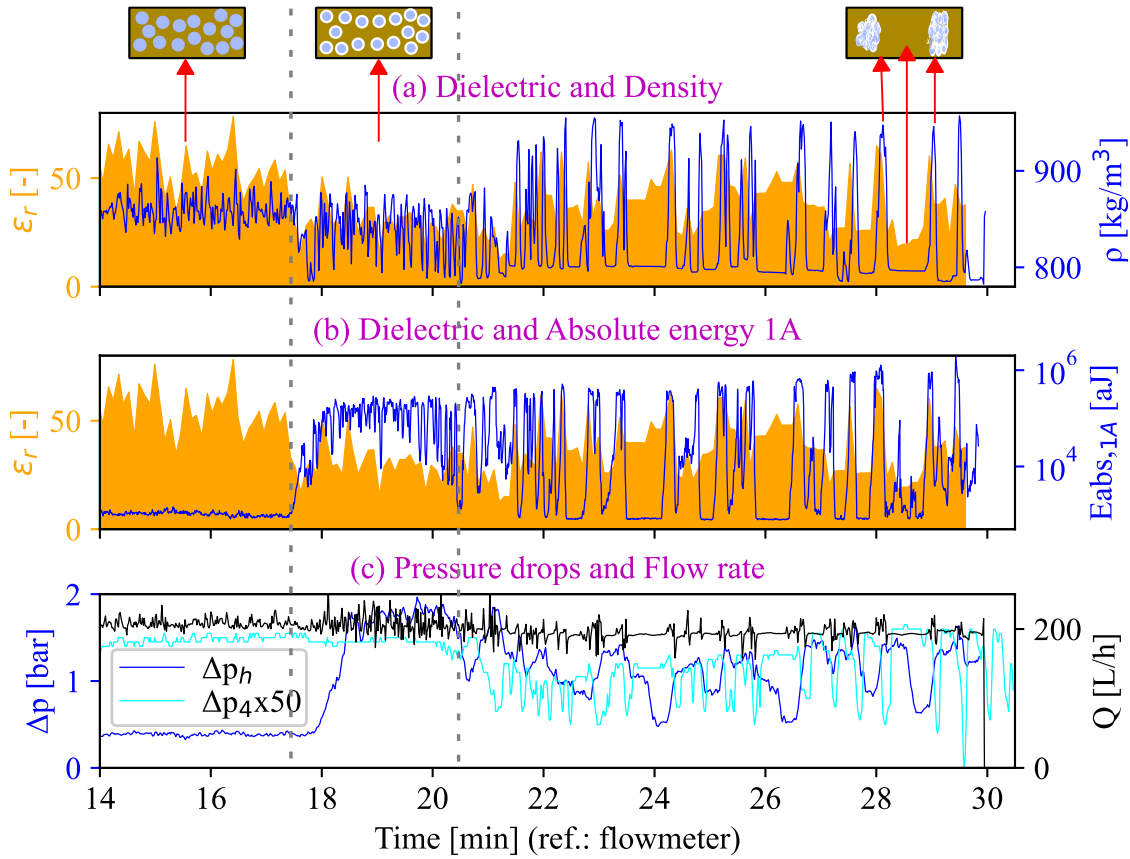
238 239 Figure 5. Experiment at 30% water-cut and 200 L/h (#1 in Table 5), showing the time evolution of (a) 240 dielectric and density, (b) dielectric and absolute energy, and (c) pressure drops and flow rate.
