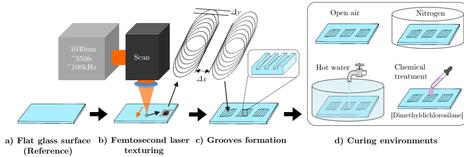
Figure 3: A schematic layout of the femtosecond laser processing system and curing environments. a) A sketch of the reference glass slide. b) A diagram explaining the production of grooves by femtosecond laser texturing following the scan path shown with \Delta x and \Delta y . c) The depth and periodicity of the grooves are dependent on the laser parameters used in their creation. d) Each textured glass slide was replicated to be cured in four different chemical environments.
