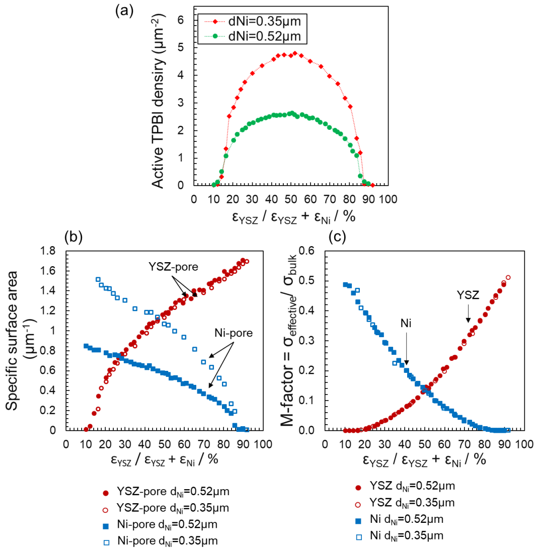
Fig. 5. Evolution of (a) active TPBI density, (b) Ni-pore and YSZ-pore specific surface area and (c) YSZ and Ni M-factors as a function of the volume fraction of YSZ in the solid phase for the two sets of microstructure ( d_{\text{Ni}}=0.35\mu\text{m} and d_{\text{Ni}}=0.52\mu\text{m} ).
