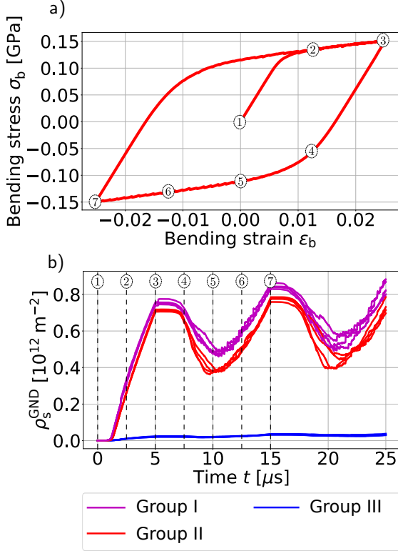
Figure 7: CDD simulation of bi-directional bending. (a): Cycle of bending moment based on the displacement driven loading and (b): resulting GND density evolution for the 12 different slip systems grouped according to Sec. 2.
