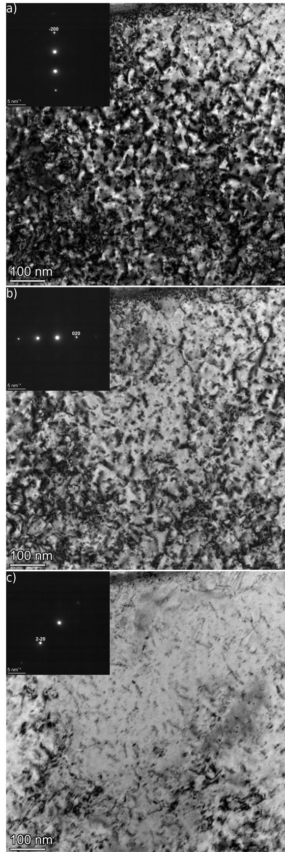
Supplementary Figure S3: TEM results. a) BF in (200), b) (020), c) (2 \bar{2} 0) two-beam conditions.
