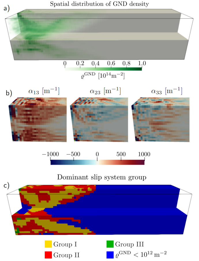
Figure 9: Distribution of GNDs at stage 7 of the CDD simulations. (a): The spatial distribution of the GND density, (b): contour plots of the tensor components \alpha_{i3} and (c): the dominant slip system groups over the cantilever beam.
