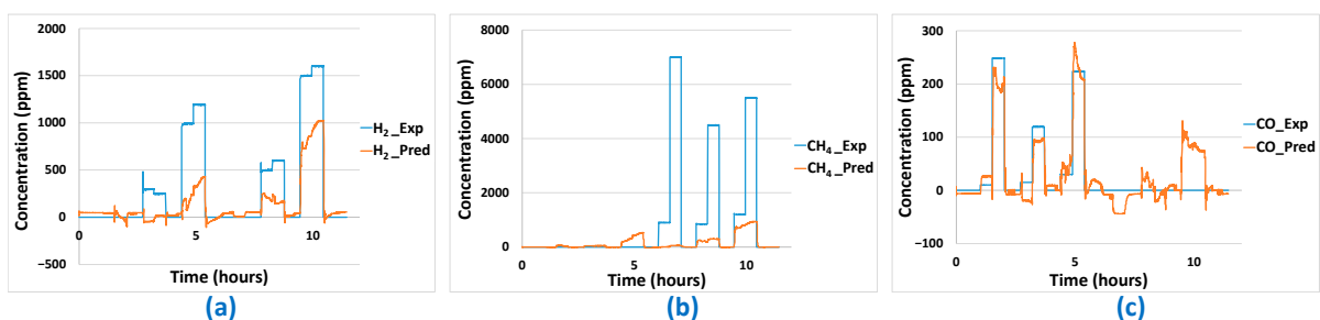
Figure 18. Gas concentration predictions ( _{Pred} in the legend) on aged sensor platform for: (a) H_2 , (b) CH_4 , (c) CO using the previously developed ANN model—comparison to experimental used concentrations ( _{Exp} in the legend).
