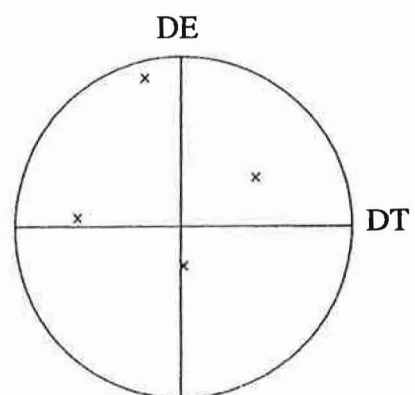
Grain 19 ( S^-_{DL} )
