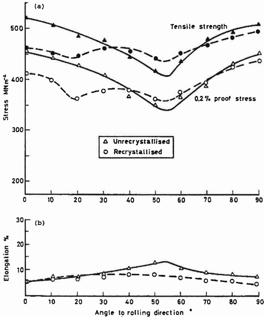
a yield and tensile strength; b elongation
